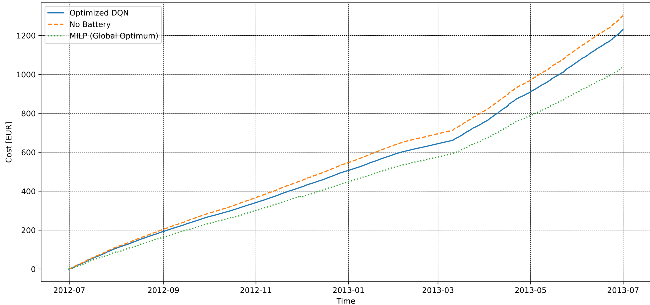
User 5 - Extended Convergence - Electricity Cost [DQN vs MILP]
